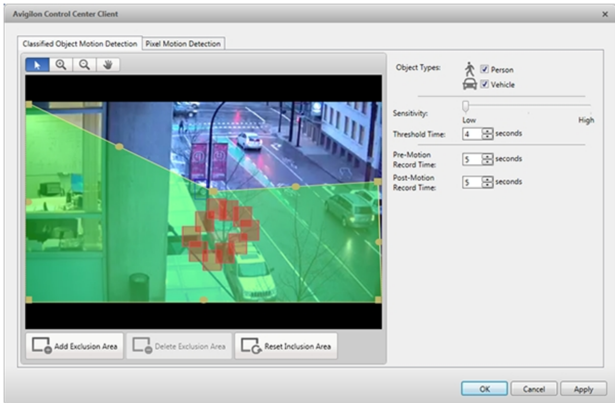
Figure 6: The Motion Detection dialog box: the Classified Object Motion Detection tab
